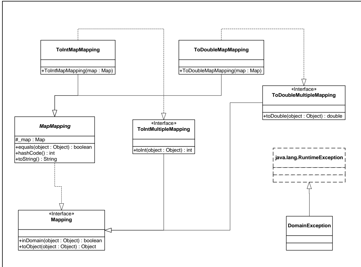
FIGURE 4.3. Classes in the graph.mapping package.
