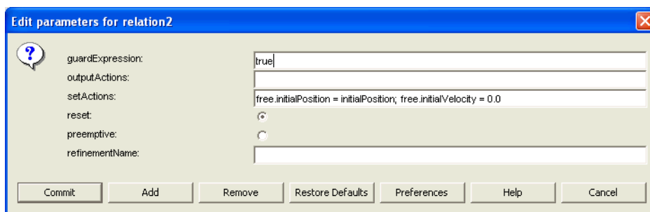
FIGURE 2.61. Transition dialog for the transition from init to free in figure 2.55.
