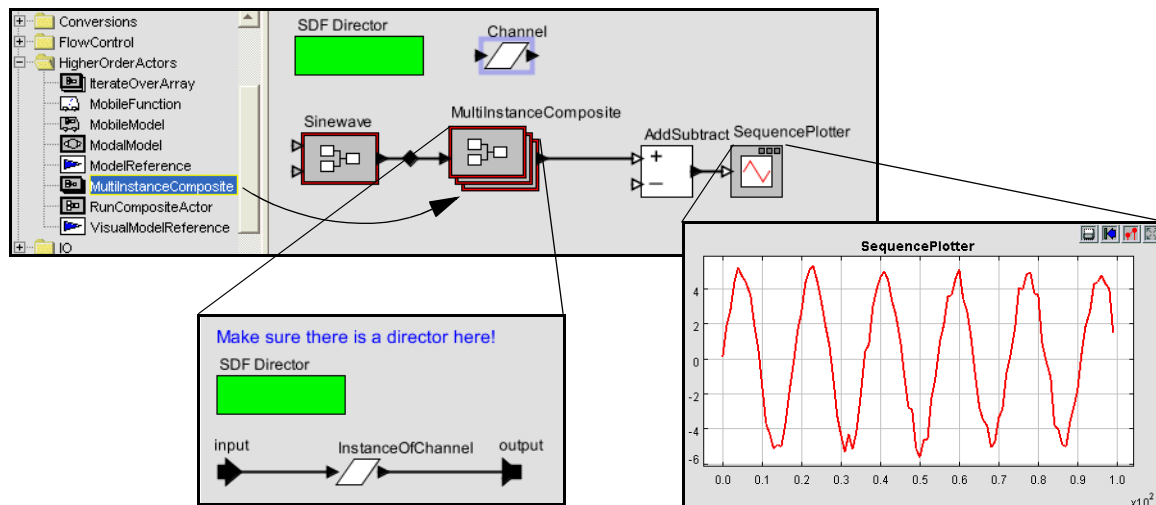
FIGURE 2.45. A model that is equivalent to that of figure 2.37, but using a MultiInstanceComposite, which permits the number of instances of the channel to change by simply changing one parameter value.
