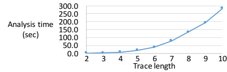
Figure 14: Verification times on the Auth model.
