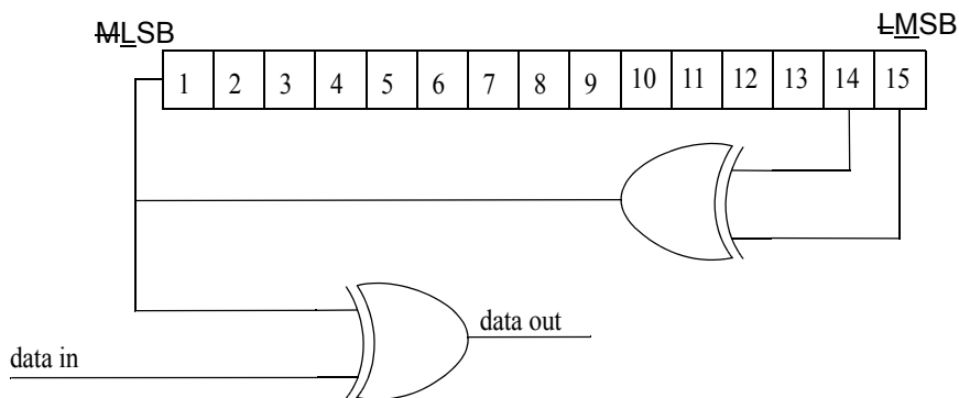
Figure 197—PRBS generator for data randomization
