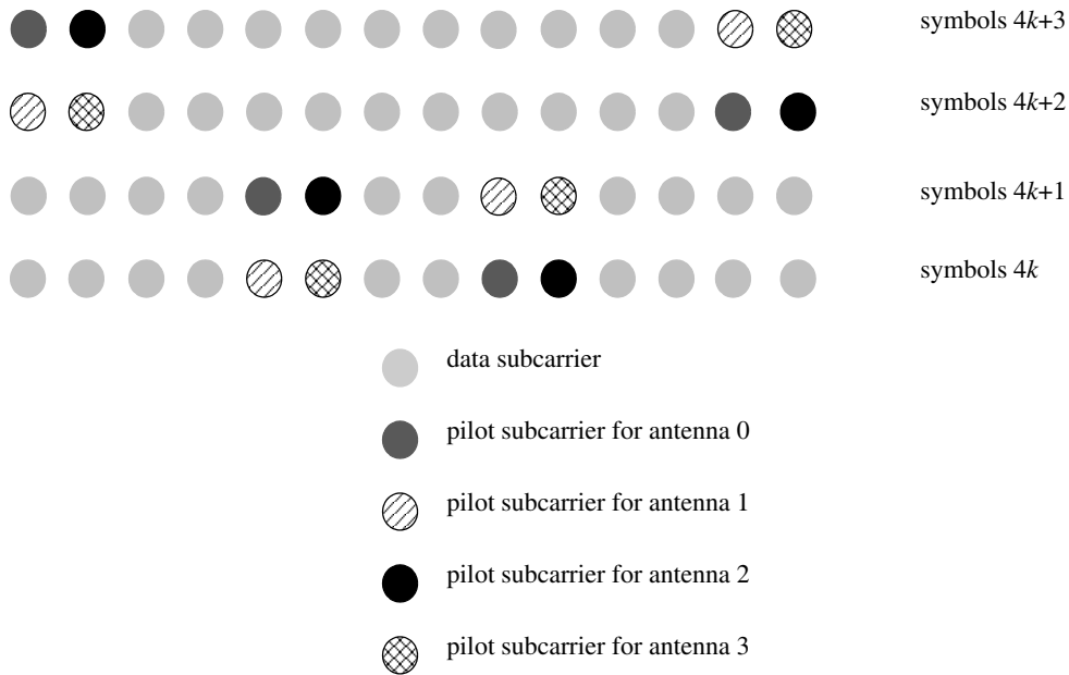
Figure 251—Cluster structure for STC PUSC using 4 antennas
