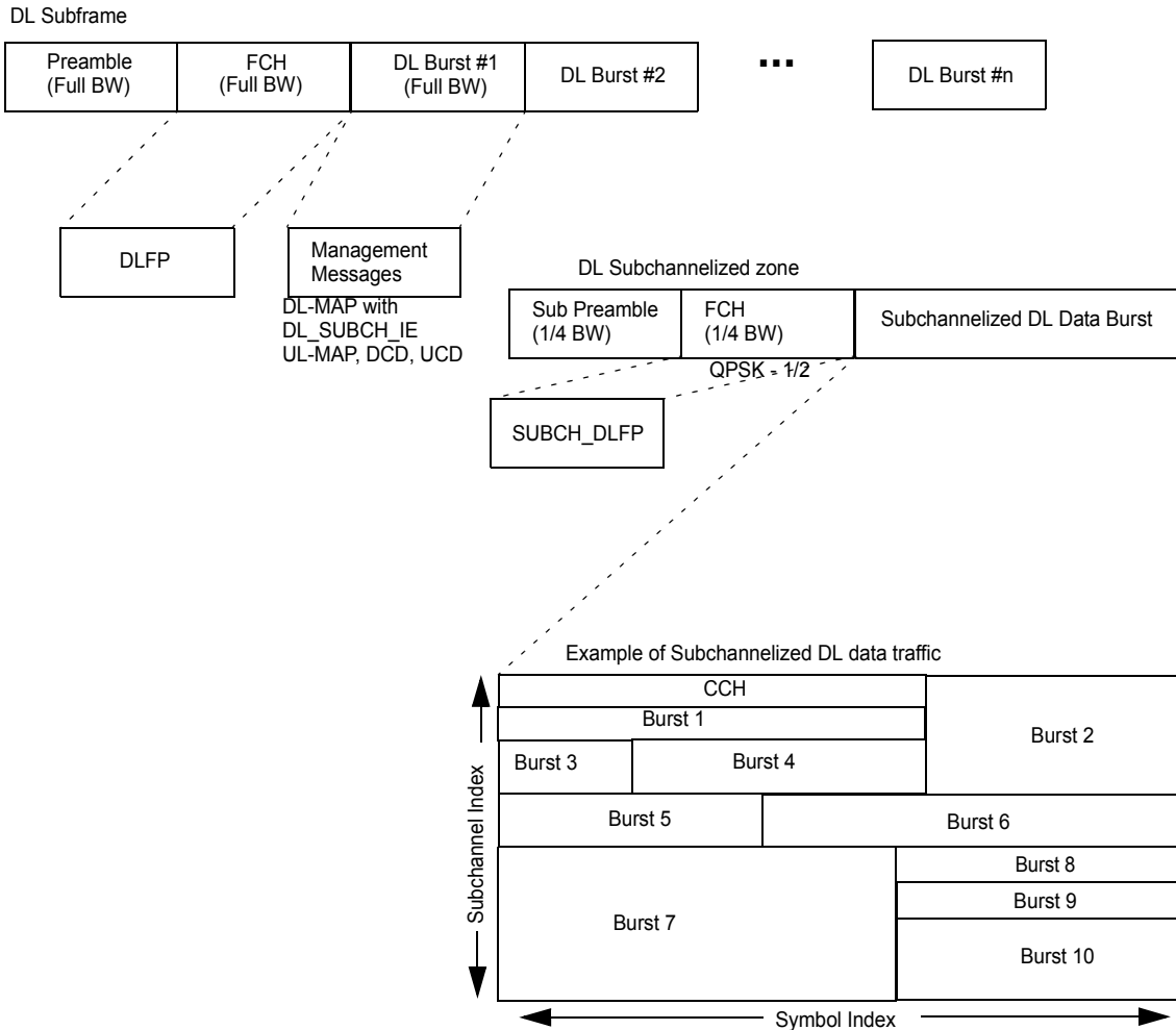
Figure 208a—Format of DL subchannelization zone
