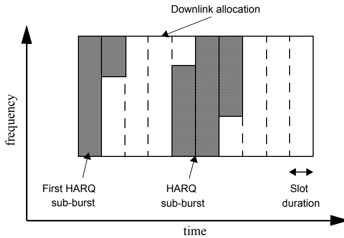
Figure 229c—HARQ downlink allocation
