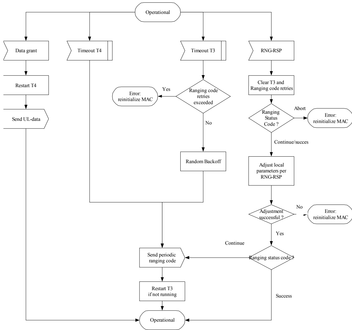
Figure 90—Periodic CDMA ranging—SS
