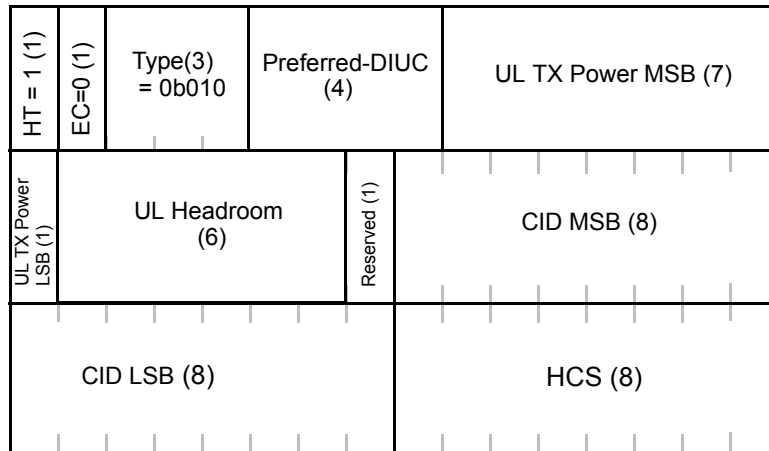
Figure 20d—PHY channel report header
