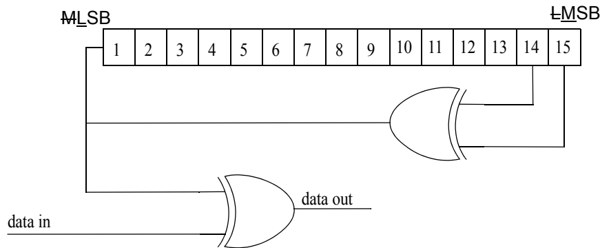
Figure 260—PRBS generator of the randomization
