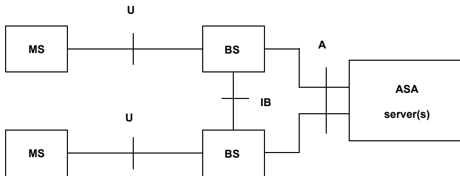
Figure G.2—Logical network reference model, control plane
