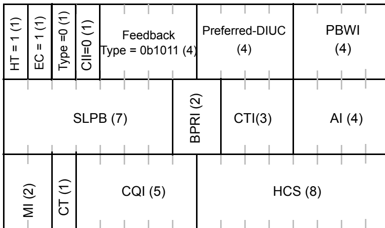
Figure 20k—MIMO Channel Feedback header without CID field
