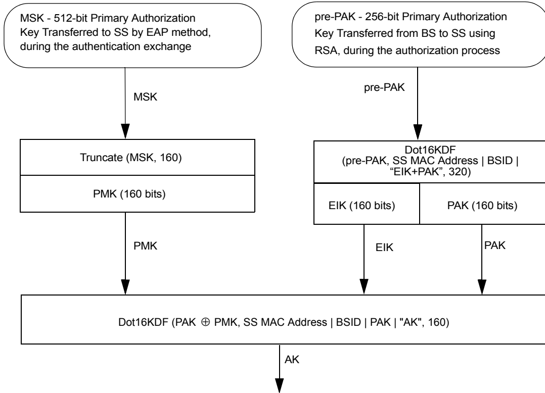
Figure 130l—AK from PAK and PMK (RSA-based and EAP-based authorization)
