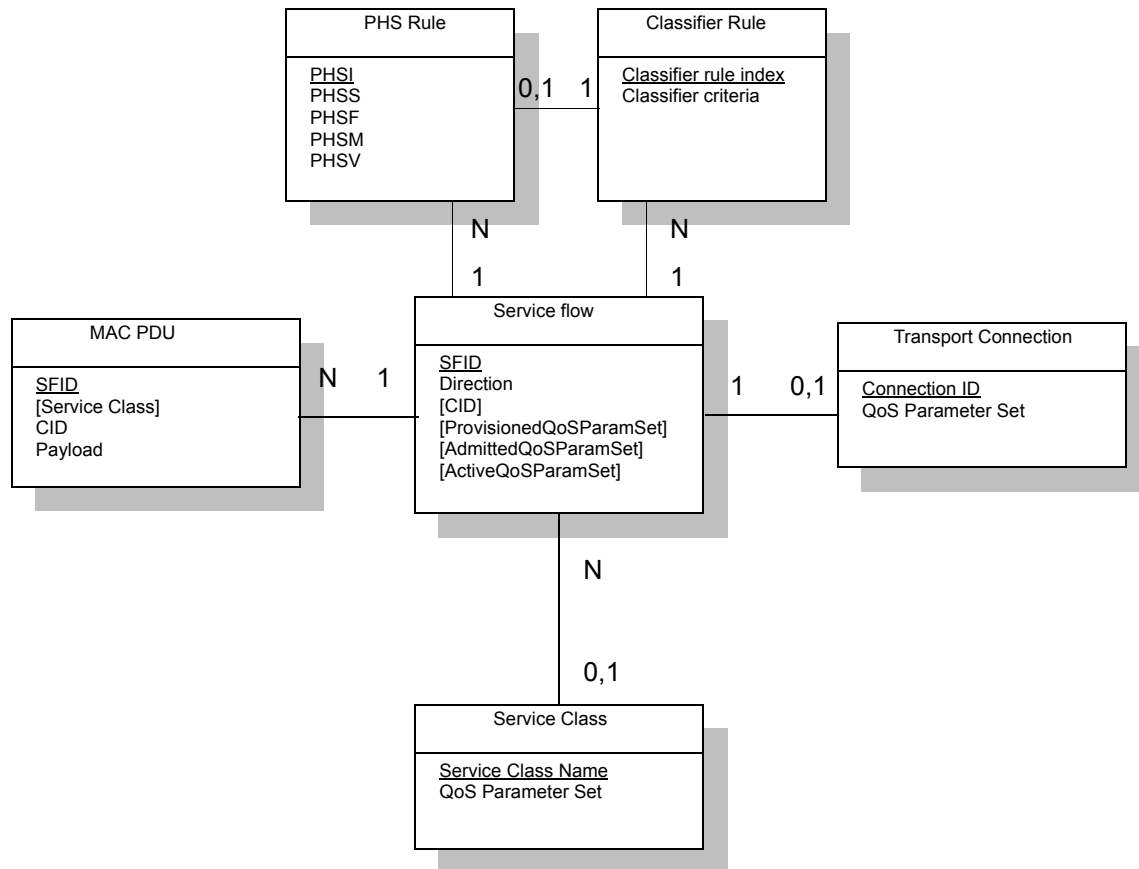
Figure 95—Theory of Operation Object Model
