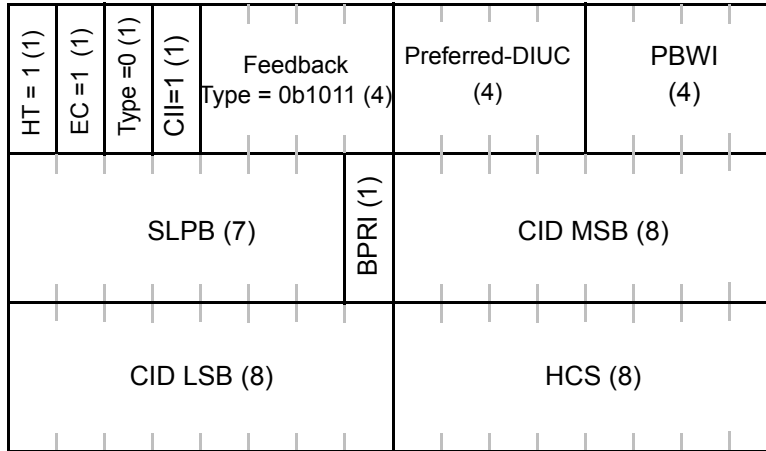
Figure 20j—MIMO Channel Feedback header with CID field
