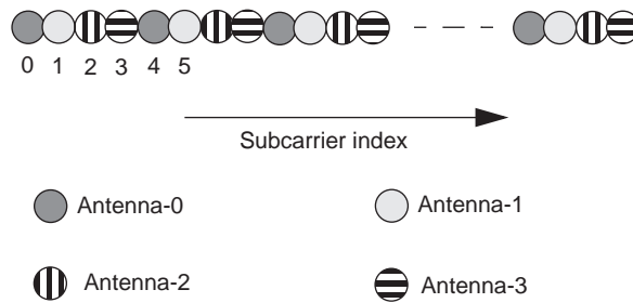
Figure 251n—Midamble FUSC structure (frequency domain)
