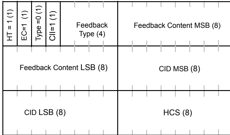
Figure 20h— Feedback header with CID field
