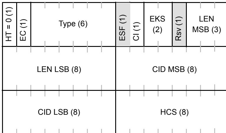
Figure 19—Generic MAC header format
