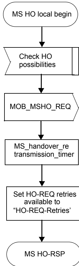
Figure 130d—MS initiating handover with the BS
