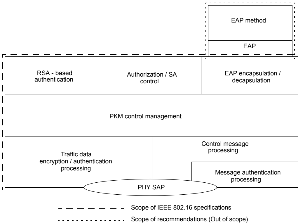
Figure 130j—Security sublayer
