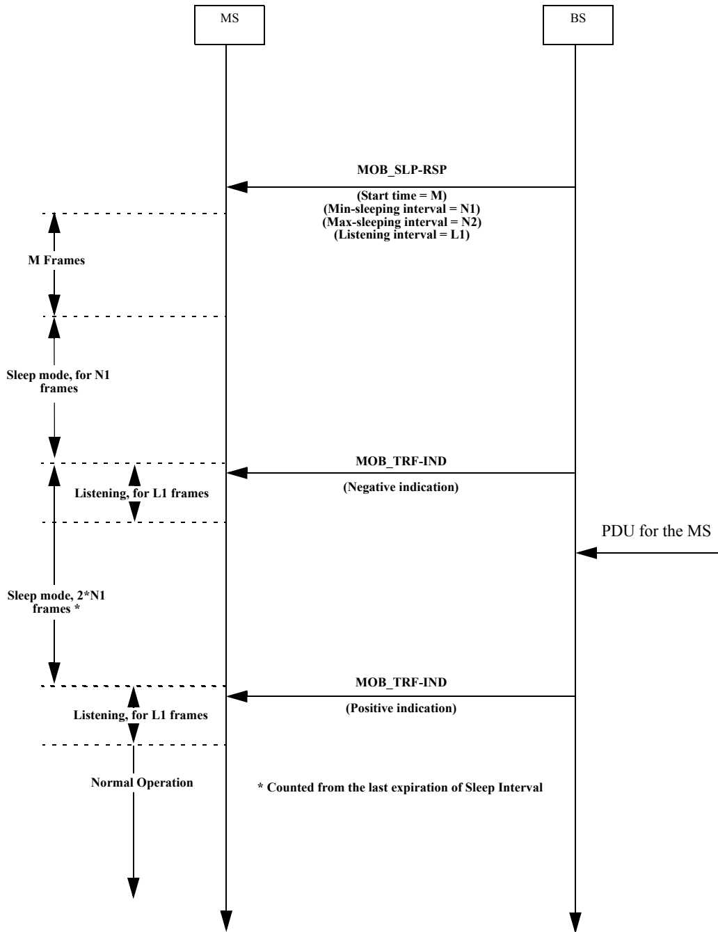
Figure D.8—Example sleep mode — BS initiated
