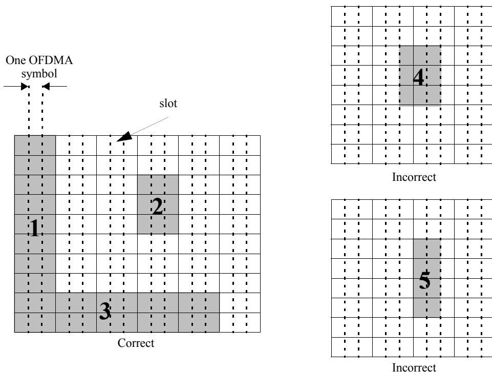
Figure 222a—Example of rectangular allocation rules
