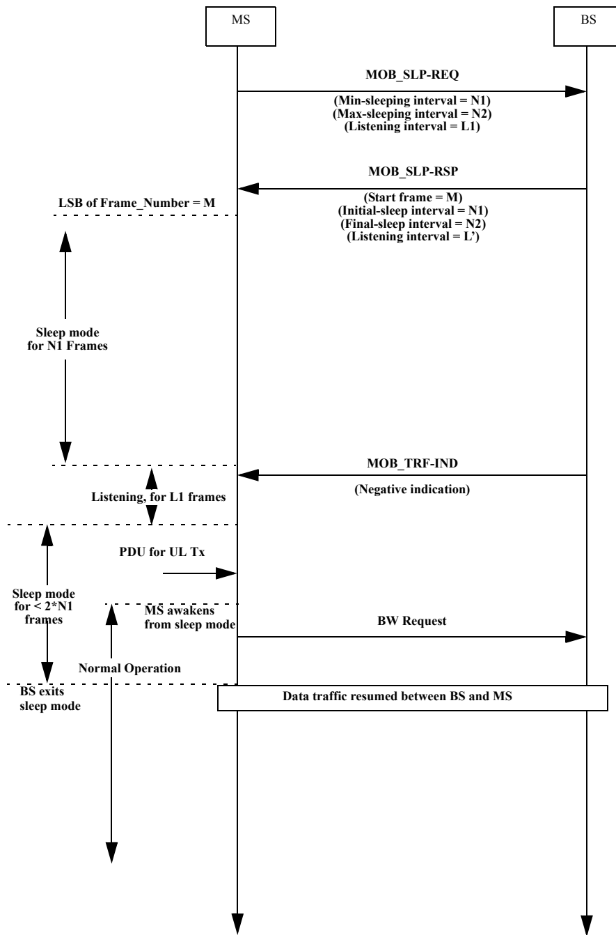
Figure D.9—Sleep mode—MS initiating awakening
