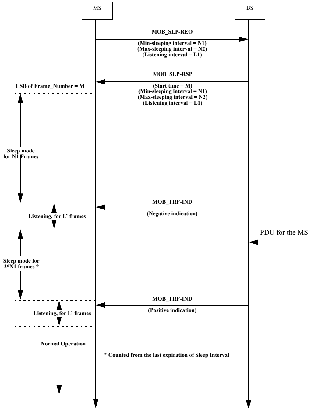
Figure D.7—Example sleep mode — MS initiated
