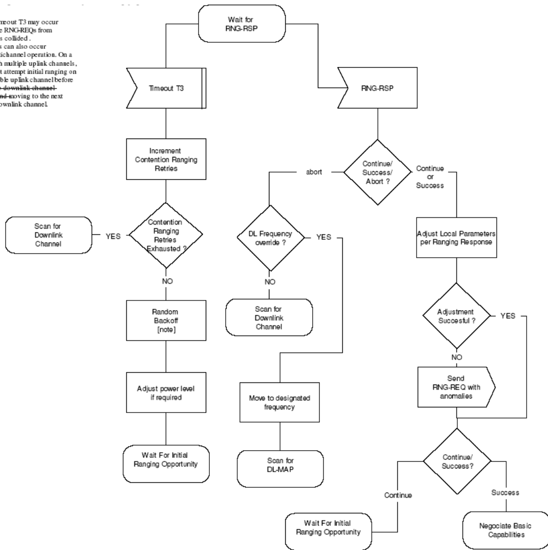
Figure 61 – Initial Ranging – SS (part 2)
