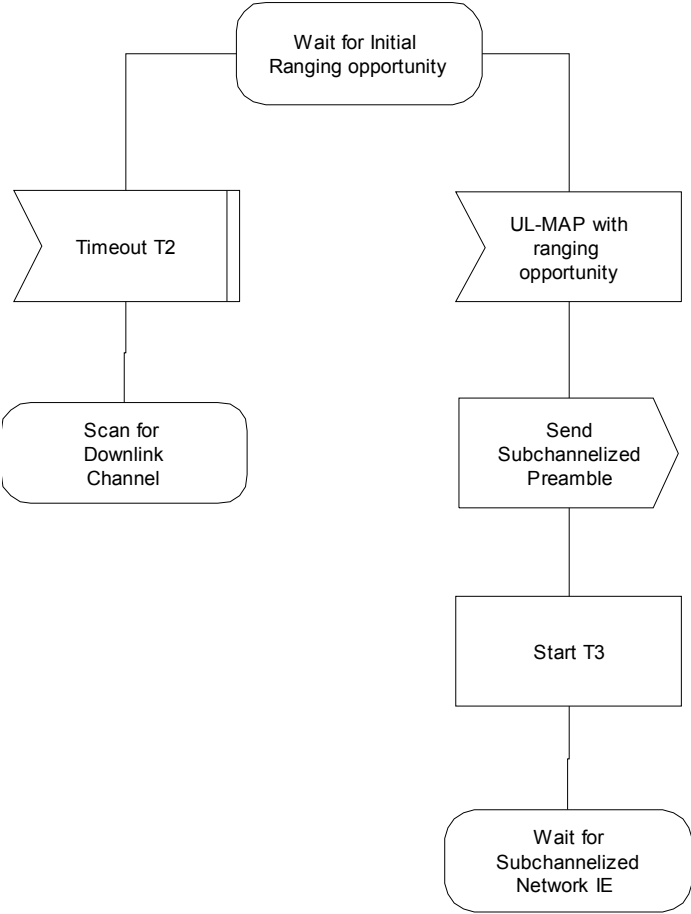
Figure 210a—Subchannelized Initial Ranging—SS (part 1a)
