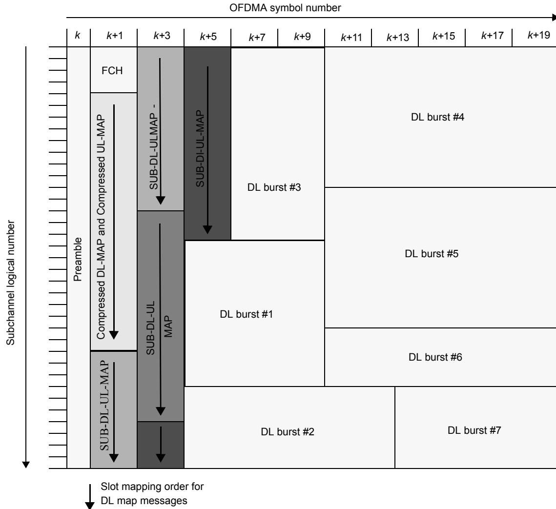
Figure 23b—Sub-MAP Burst
