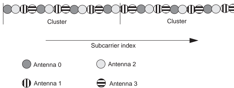
Figure 251o—Midamble PUSC structure (frequency domain)
