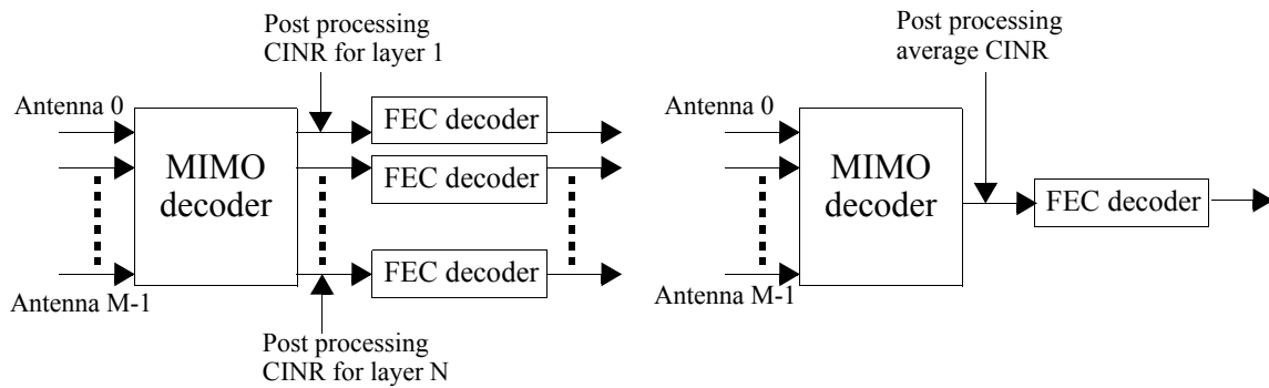
Figure 230a—Post processed CINR for MIMO region
