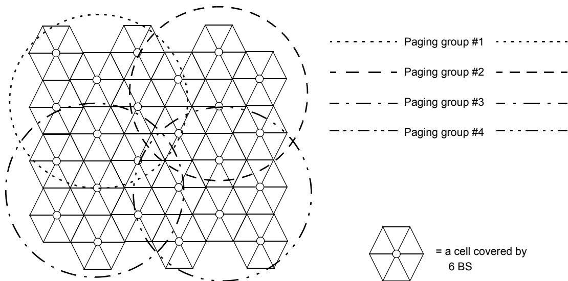
Figure 130i—Paging-groups example
