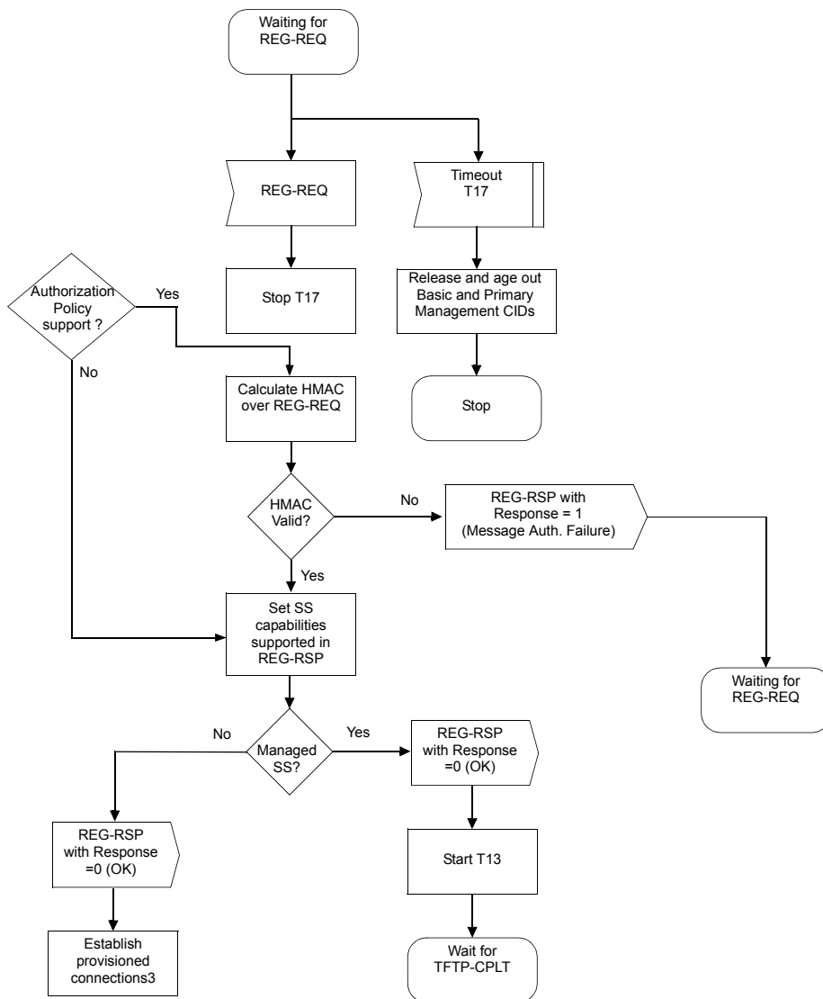
Figure 70—Registration—BS
