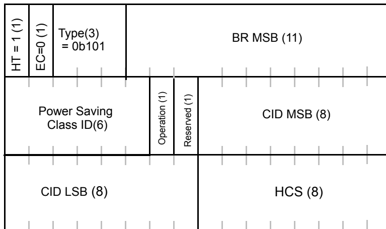
Figure 20e—Bandwidth request and uplink sleep control header
