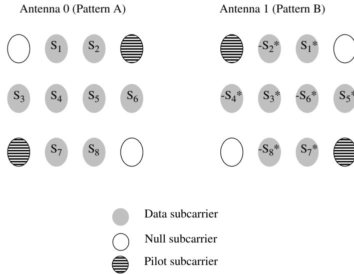
Figure 249—Mapping of data subcarriers in STTD mode
