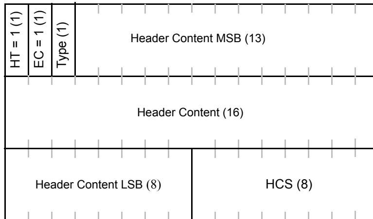
Figure 20g—MAC signaling header type II format
