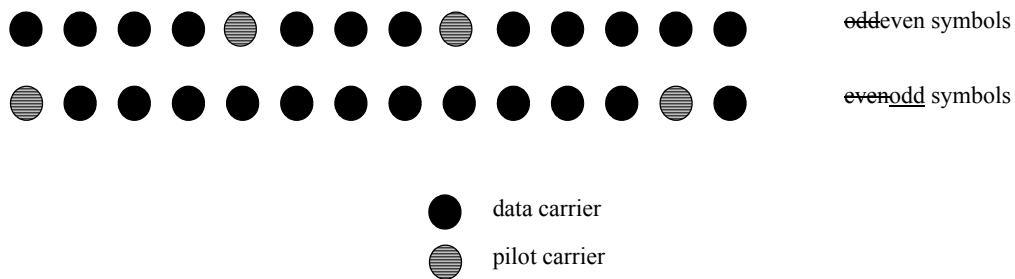
Figure 234—Cluster structure
