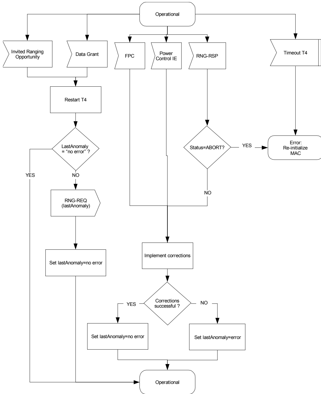
Figure 84—Periodic Ranging—SS
