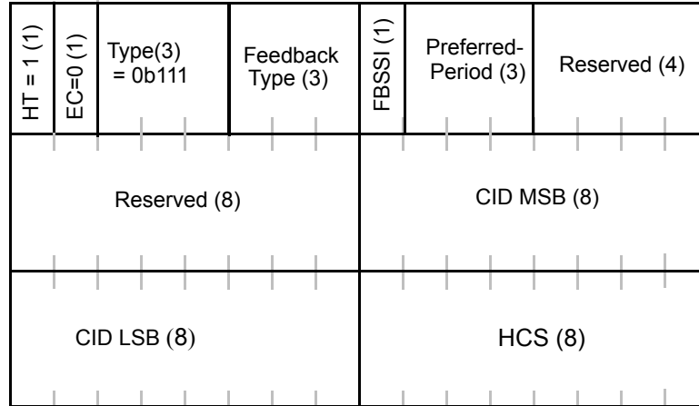
Figure 20c— CQICH allocation request
