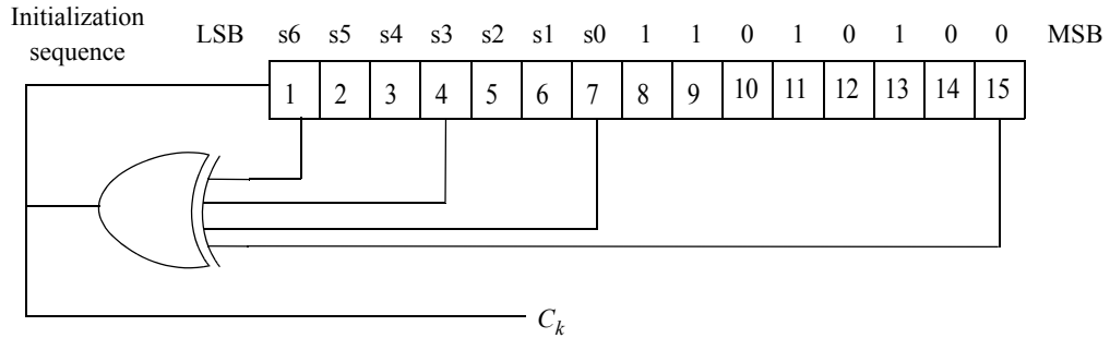
Figure 243—PRBS generator for ranging code generation
