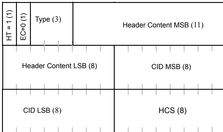
Figure 19a—MAC signaling header type I format
