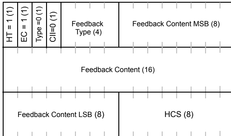
Figure 20i—Feedback header without CID field
