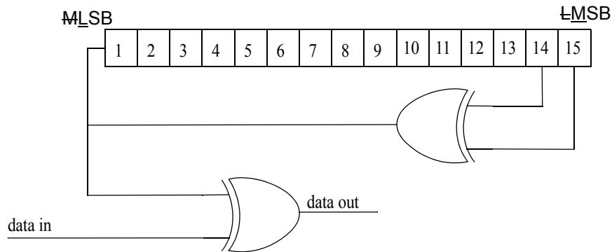
Figure 253—PRBS generator for data randomization
