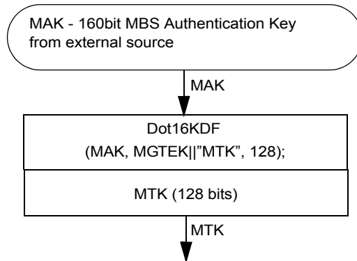
Figure 130p—MTK key derivation from MAK
