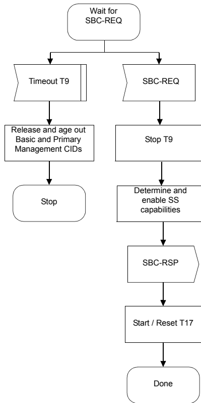
Figure 67—Negotiate Basic Capabilities—BS
