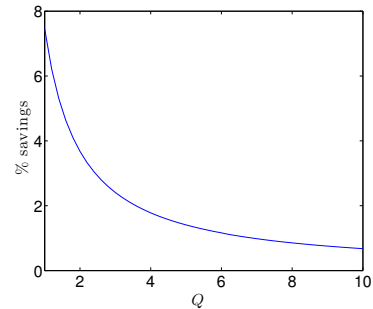
Fig. 1. p = 4 , percent savings using pricing scheme plotted against Q : \hat{R} .
