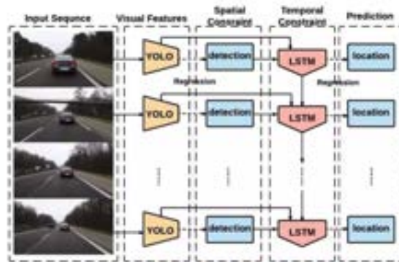
Figure 1.4: Yolo with LSTM diagram
