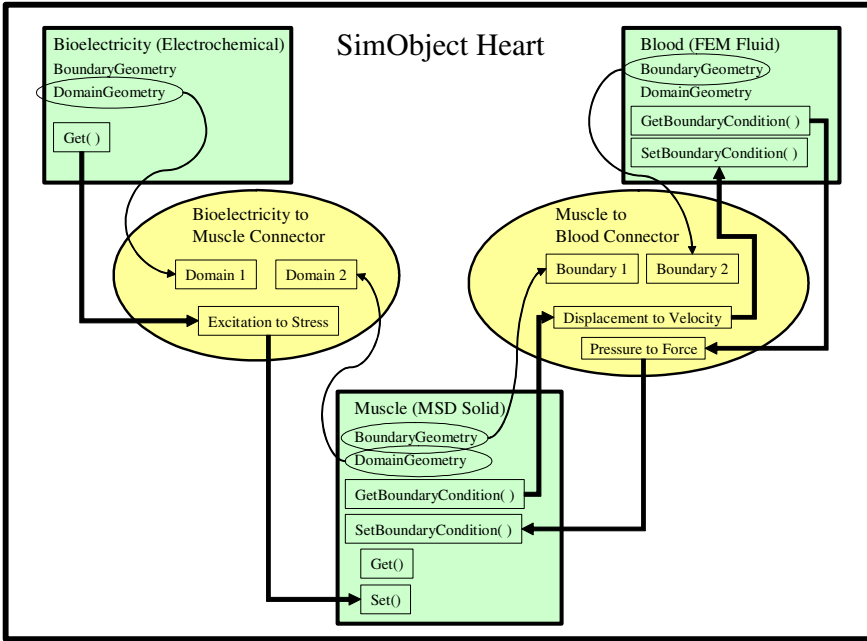
Fig. 3. Connector class example.
