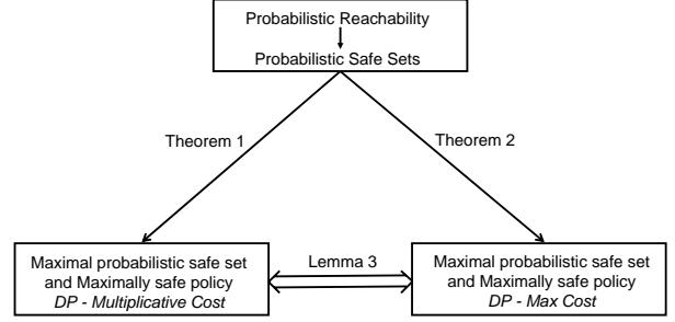
Fig. 1. Dual interpretation of the probabilistic reachability and safety problem.
