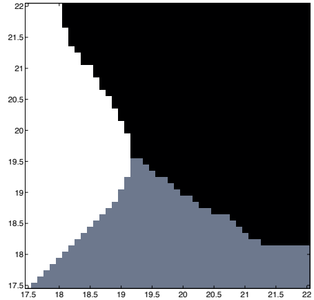
Fig. 4. Value taken by the maximally safe transition input at time k = 0 over the set of desired temperatures, when the heating system is in the OFF mode. The temperature of room 1 is reported on the horizontal axis, and that of room 2 on the vertical axis. The colors black , white , and grey respectively stand for the transition input command \mathbf{SW}_{\mathbf{OFF}} , \mathbf{SW}_1 , and \mathbf{SW}_2 .
