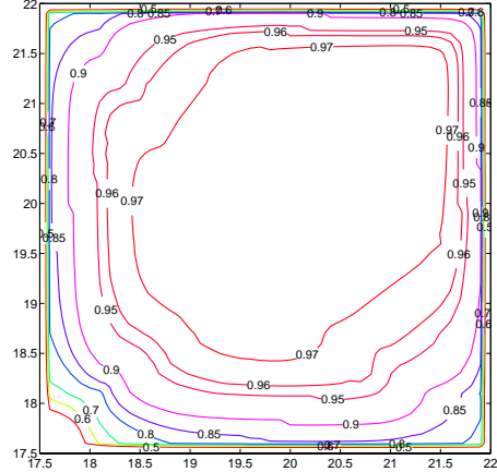
Fig. 3. Maximal probabilistic safe sets corresponding to different safety levels (0.5, 0.6, 0.7, 0.8, 0.85, 0.9, 0.95, 0.96, and 0.97) within the discrete state OFF . The temperature of room 1 is reported on the horizontal axis, and that of room 2 on the vertical axis.
