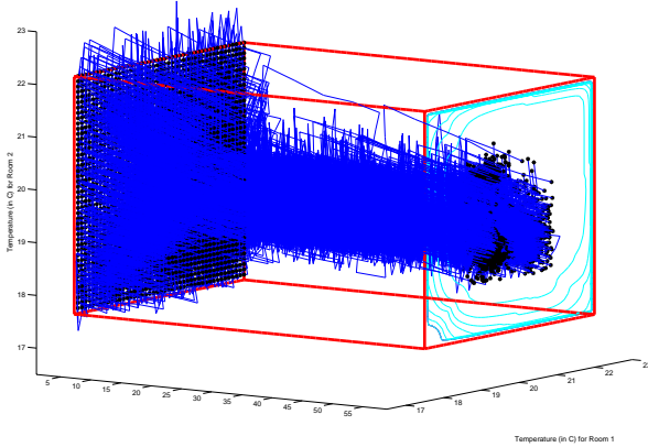
Fig. 2. Sample paths of the two rooms temperatures for executions corresponding to different initial conditions, under the same maximally safe policy.
