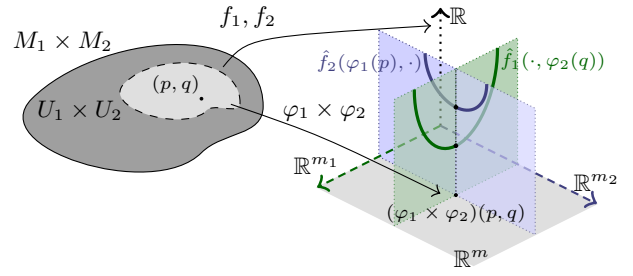
Fig. 1. The map \hat{f}_i : \mathbb{R}^m \rightarrow \mathbb{R} is the coordinate representation of f_i and it is defined by \hat{f}_i = f_i \circ (\varphi_1 \times \varphi_2)^{-1} where \varphi_1 \times \varphi_2 : U_1 \times U_2 \rightarrow \mathbb{R}^m is the coordinate map. Player i , whose cost function is f_i , can only adjust his payoff by changing his strategy in directions corresponding to \mathbb{R}^{m_i} . \hat{f}_1(\cdot, \varphi_2(q)) and \hat{f}_2(\varphi_1(p), \cdot) are slices of the coordinate representation of f_1 and f_2 , respectively.
