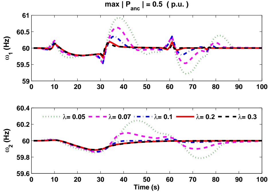
Figure 7.7: Frequency of areas 1 and 2 in response to the disturbance are shown. Prediction horizon is H = 10 and maximum ancillary power is \max|P_{\text{anc}}| = 0.5 \text{ (p.u.)} . Results are for various values of rate of change of ancillary power such that \max|\Delta P_{\text{anc}}| = \lambda .
