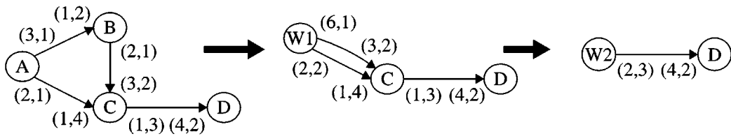
Figure 9. An MDSDF graph that has a BMLB schedule.
